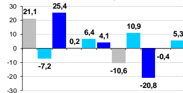
Changes - debt sec. > 1Y
