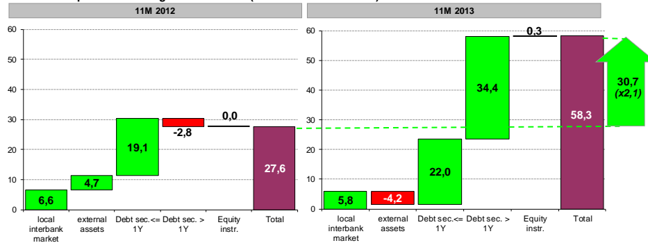
Changes - local interbank market
