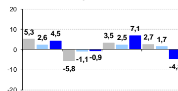
Changes - external assets
